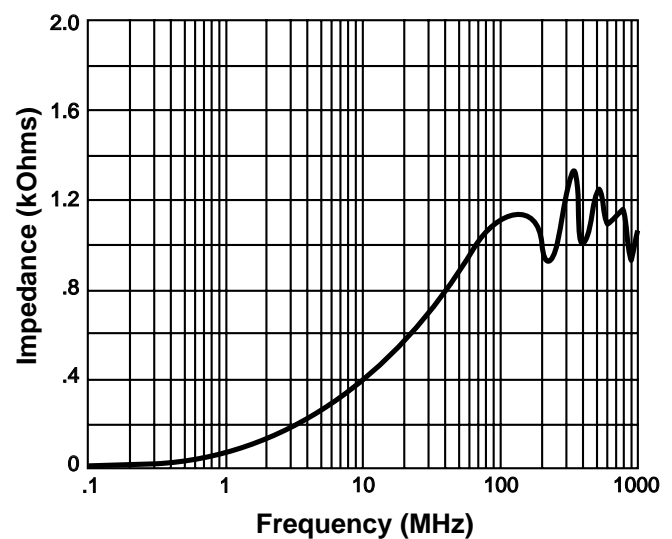
Typical Impedance
