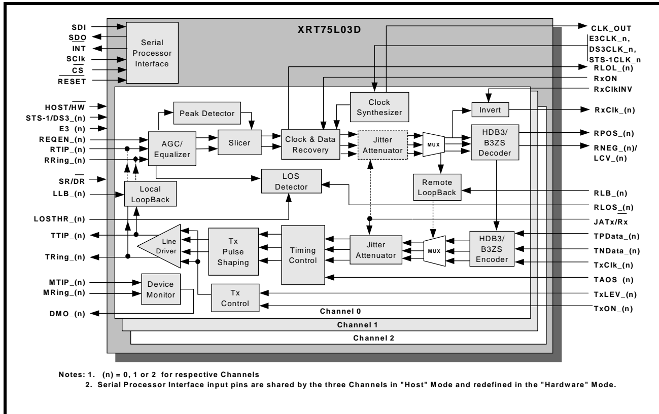
FIGURE 1. BLOCK DIAGRAM OF THE XRT75L03D
