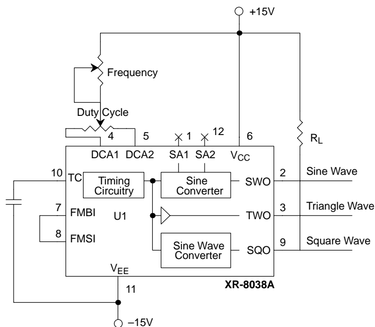
Figure 5. Single Potentiometer for External Duty Cycle Adjust
