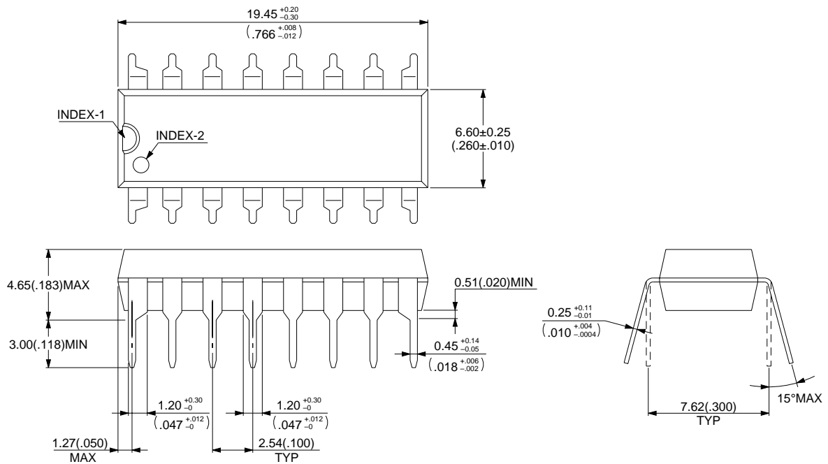
16-pin plastic DIP (DIP-16P-M03)
