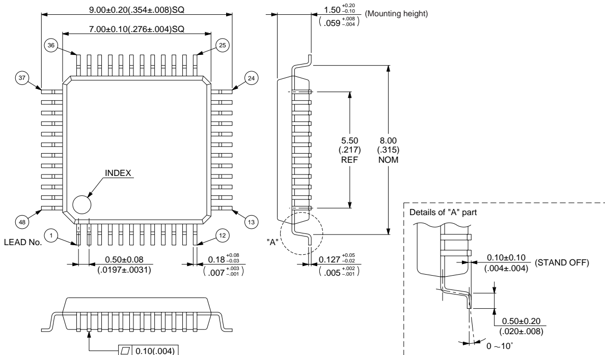
48-pin plastic LQFP (FPT-48P-M05)
