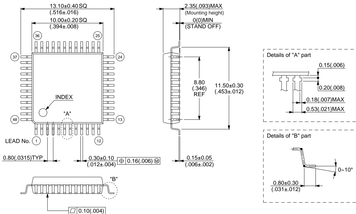
48-pin plastic QFP (FPT-48P-M13)
