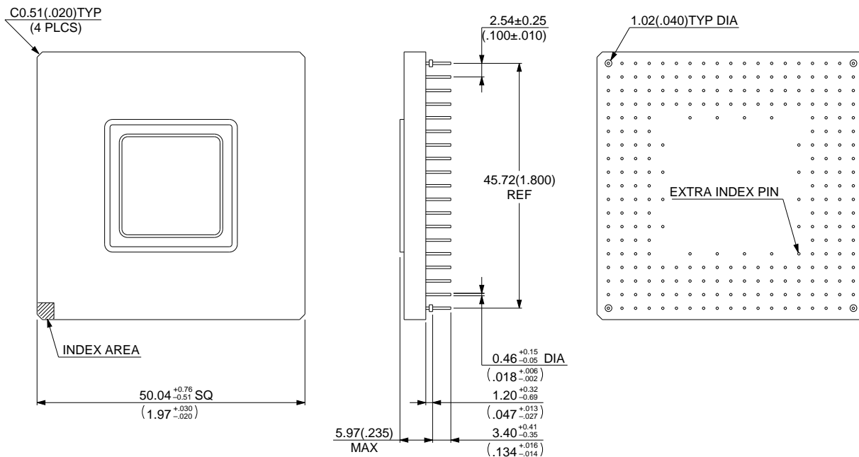
256-pin ceramic PGA (PGA-256C-A02)
