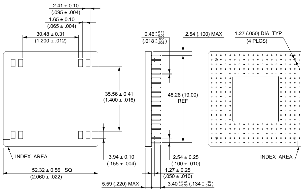
299-pin ceramic PGA (PGA-299C-A01)
