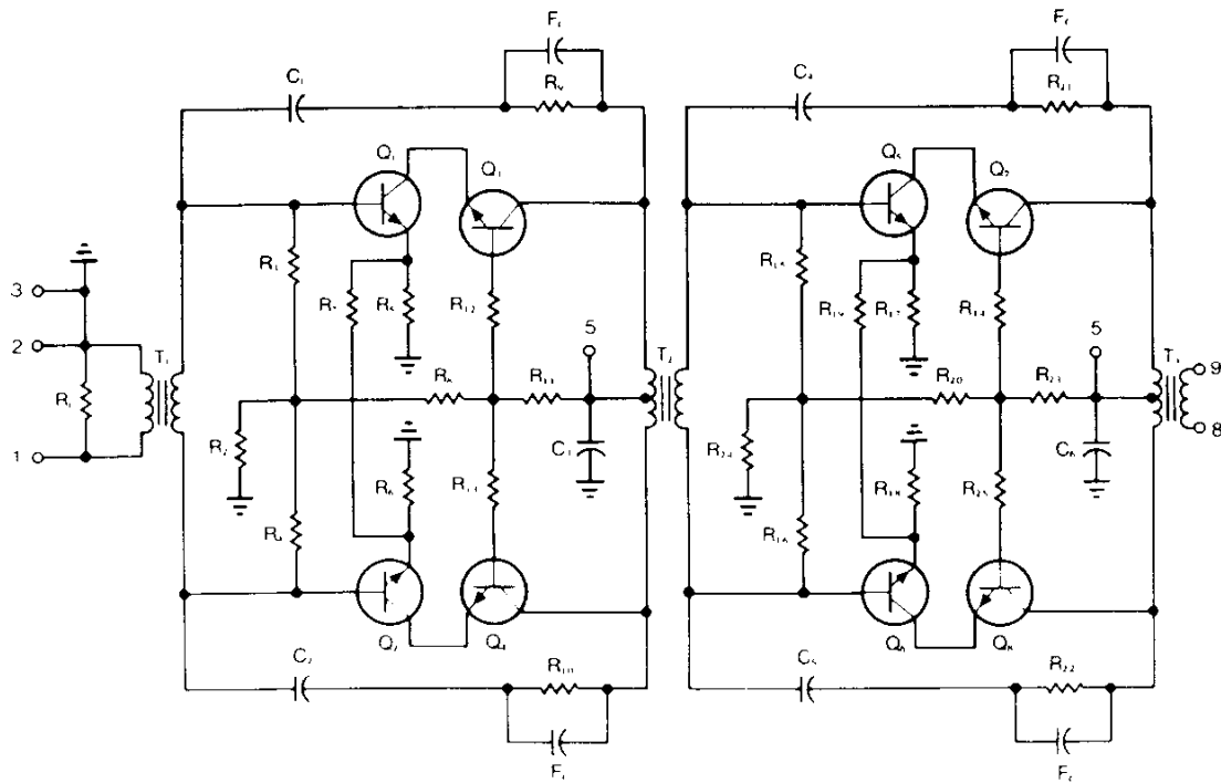
33dB Gain Block
