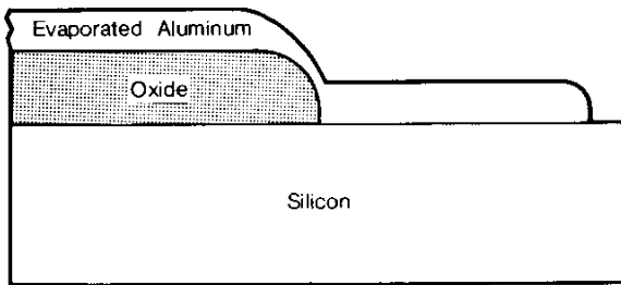
Figure 11. Oxide Step Coverage
