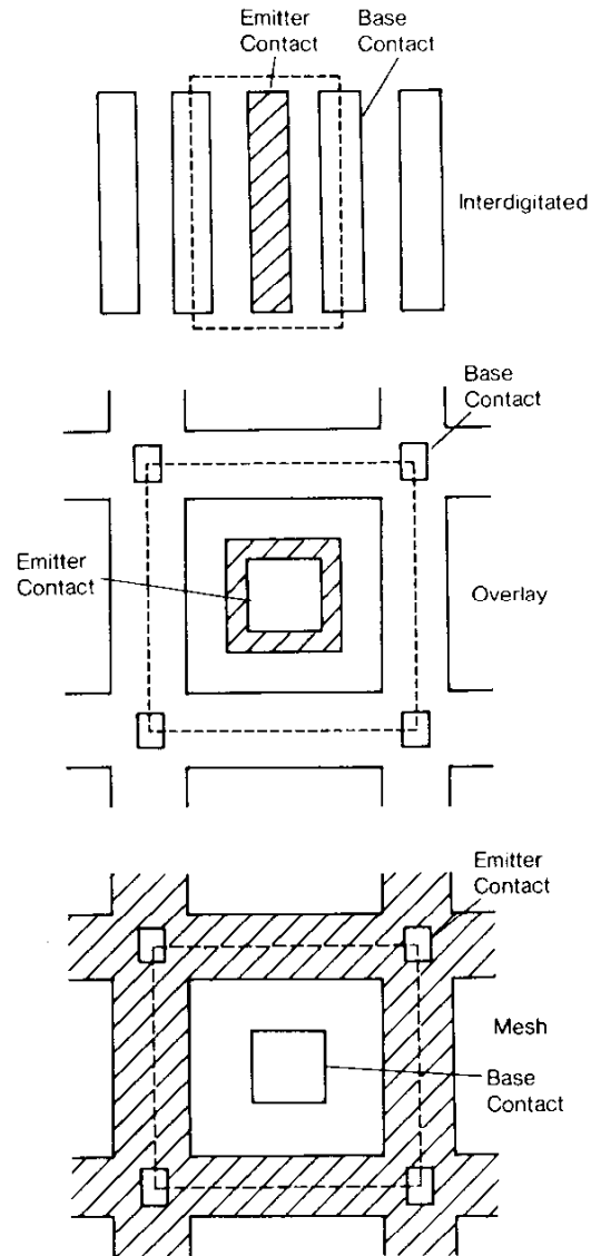
Figure 5. Typical Transistor Configurations
