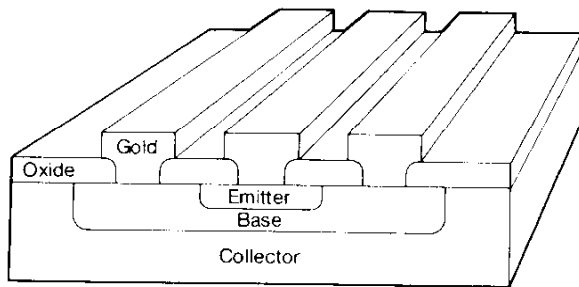
Figure 9. Transistor Metallization
