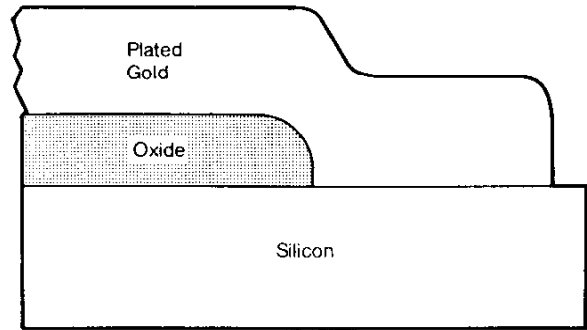
Figure 11. Oxide Step Coverage
