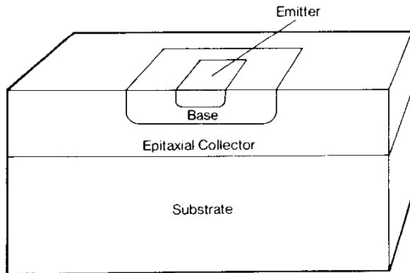
Figure 3. Planar-Epitaxial Technology
