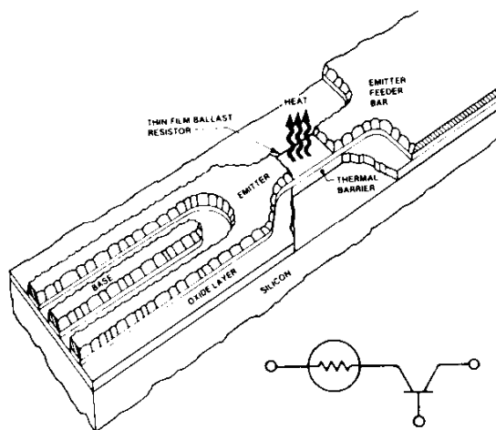
Figure 7. Ballast Resistor Configurations
