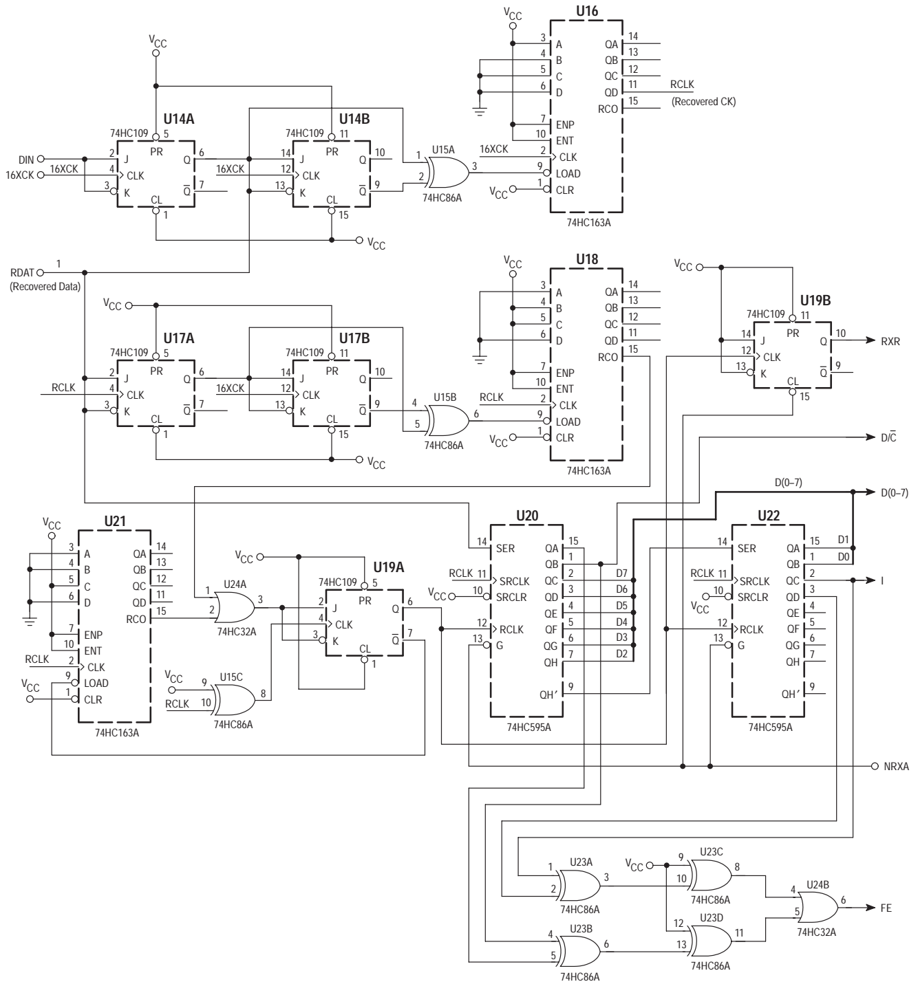
Figure 8. Decoder
