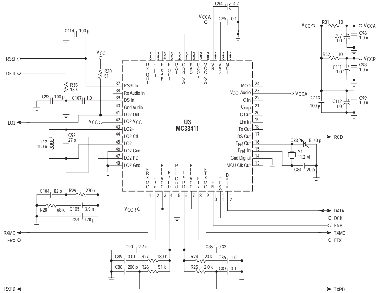
Figure 4. Baseband
