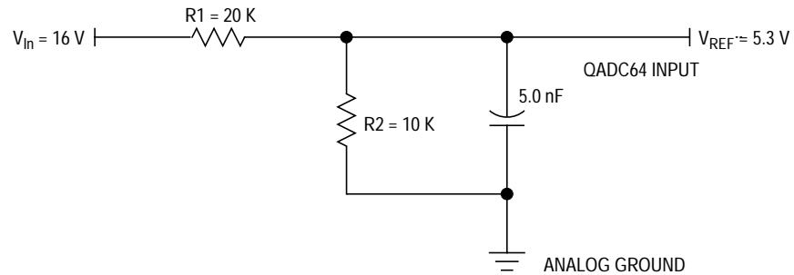
Figure 9. Conditioning a 16-Volt Input
