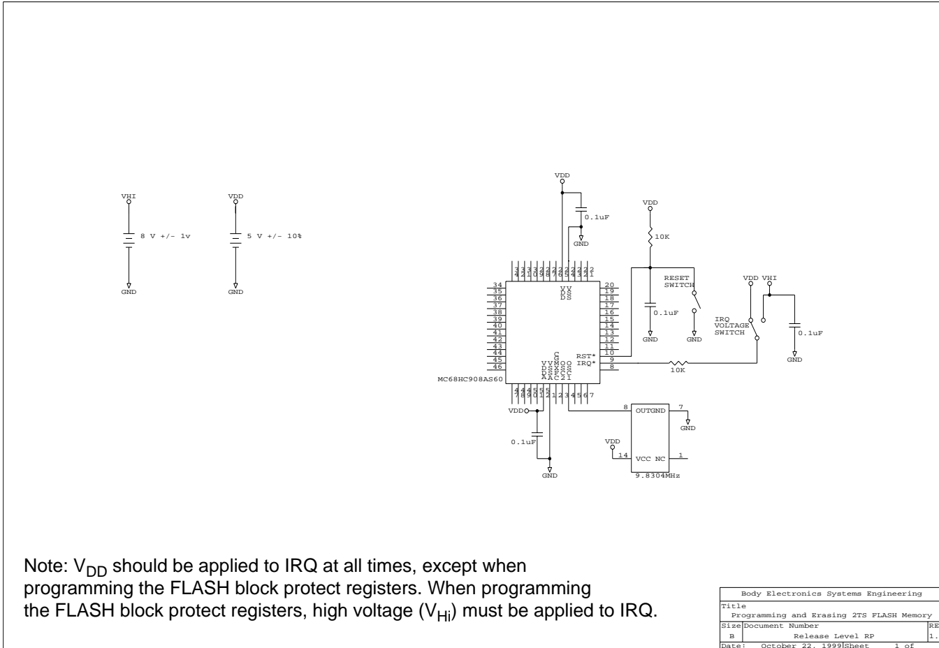
Figure 9. Hardware Schematic for Programming and Erasing FLASH 2TS on the MC68HC908AS60
