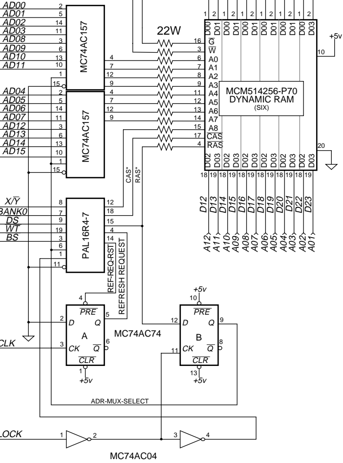
4 DSP56001-to-DRAM Schematic provides 256k words of expansion memory to the DSP56000 Application Development System.
