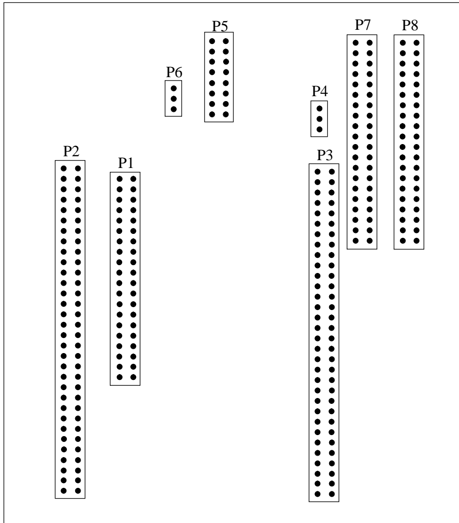
Figure 1-1. HC05L1 Emulator Module
