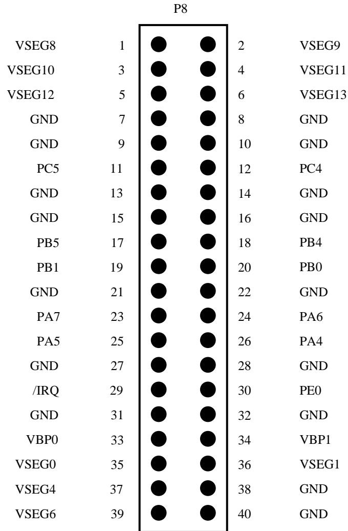
Figure 1-3. Connector P8 Pin Assignments
