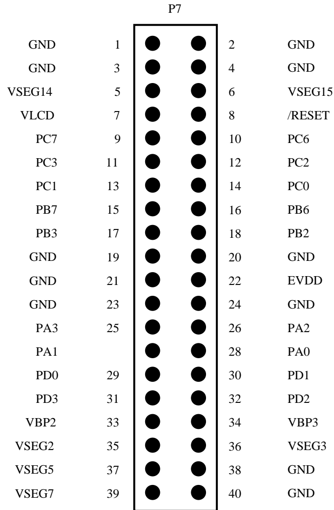
Figure 1-2. Connector P7 Pin Assignments
