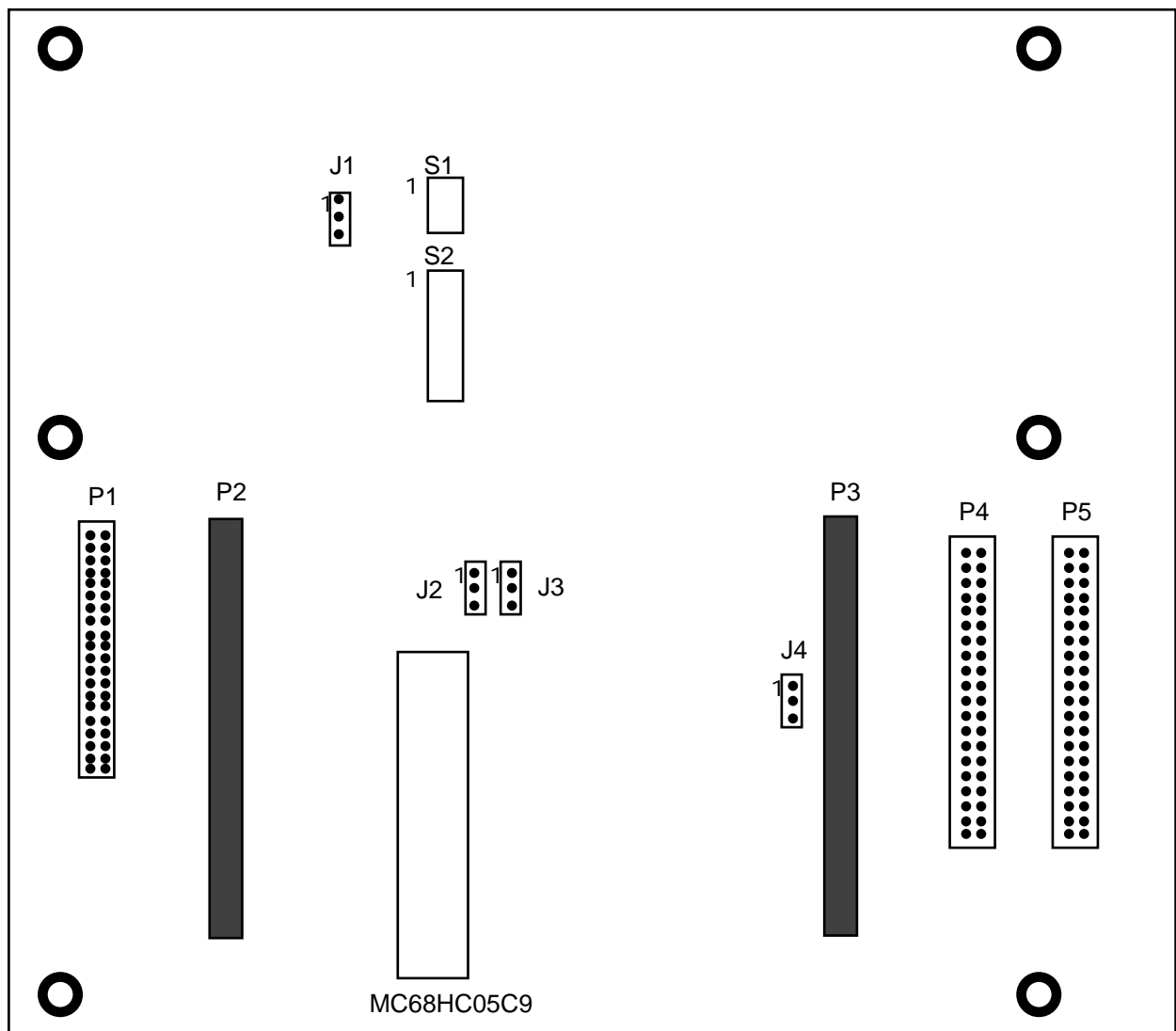
Figure 1-1. HC05D32 Emulator Module
