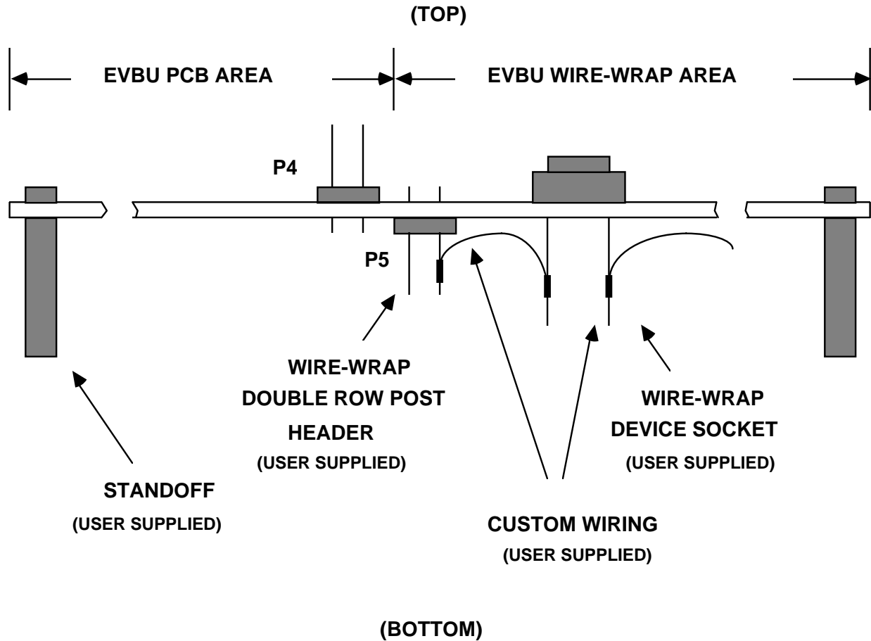
Figure 2-3. Wire-Wrap Area (Side View)
