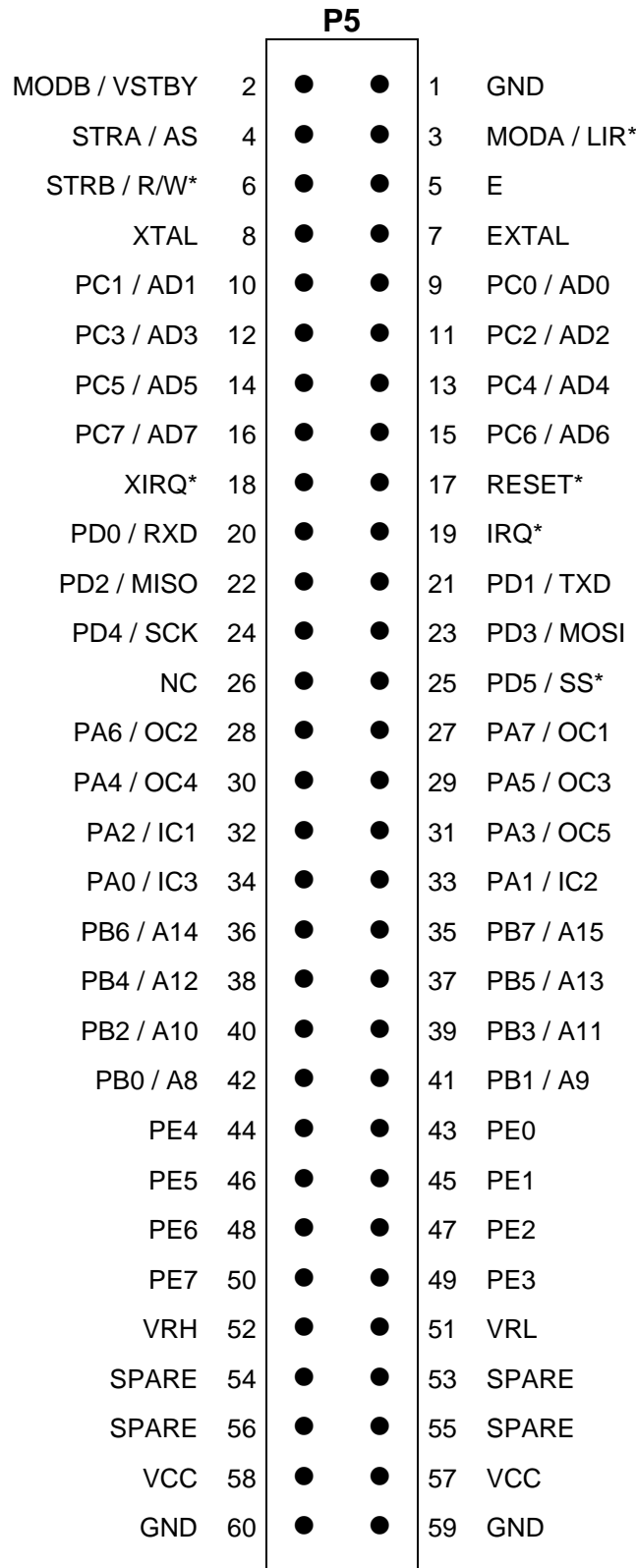
Figure 2-7. MCU I/O Port Connector P5 (EVBU Bottom View)
