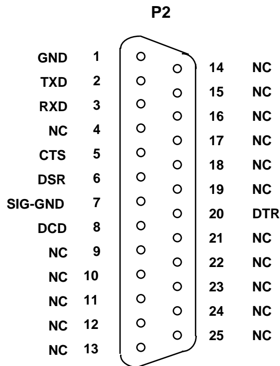
Figure 2-4. Terminal I/O Port Connector
