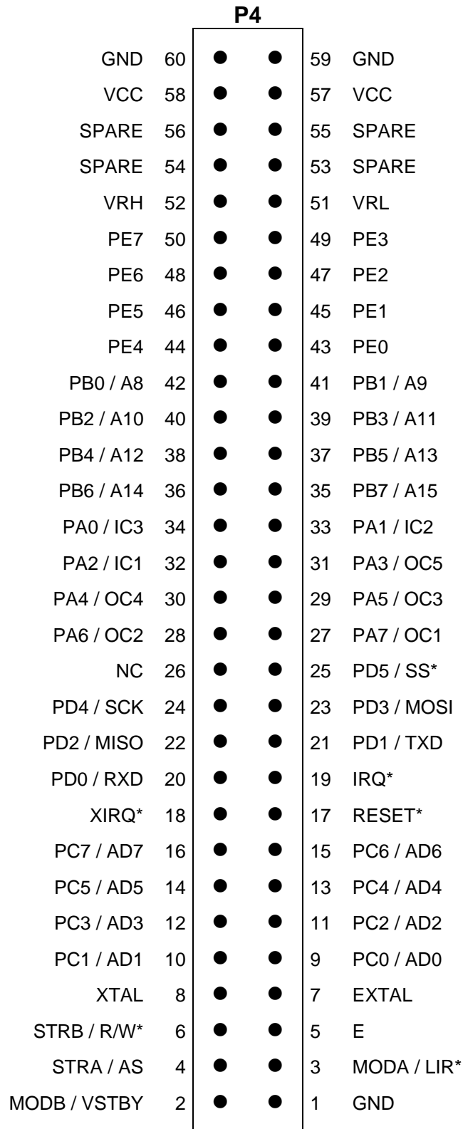
Figure 2-6. MCU I/O Port Connector P4 (EVBU Top View)
