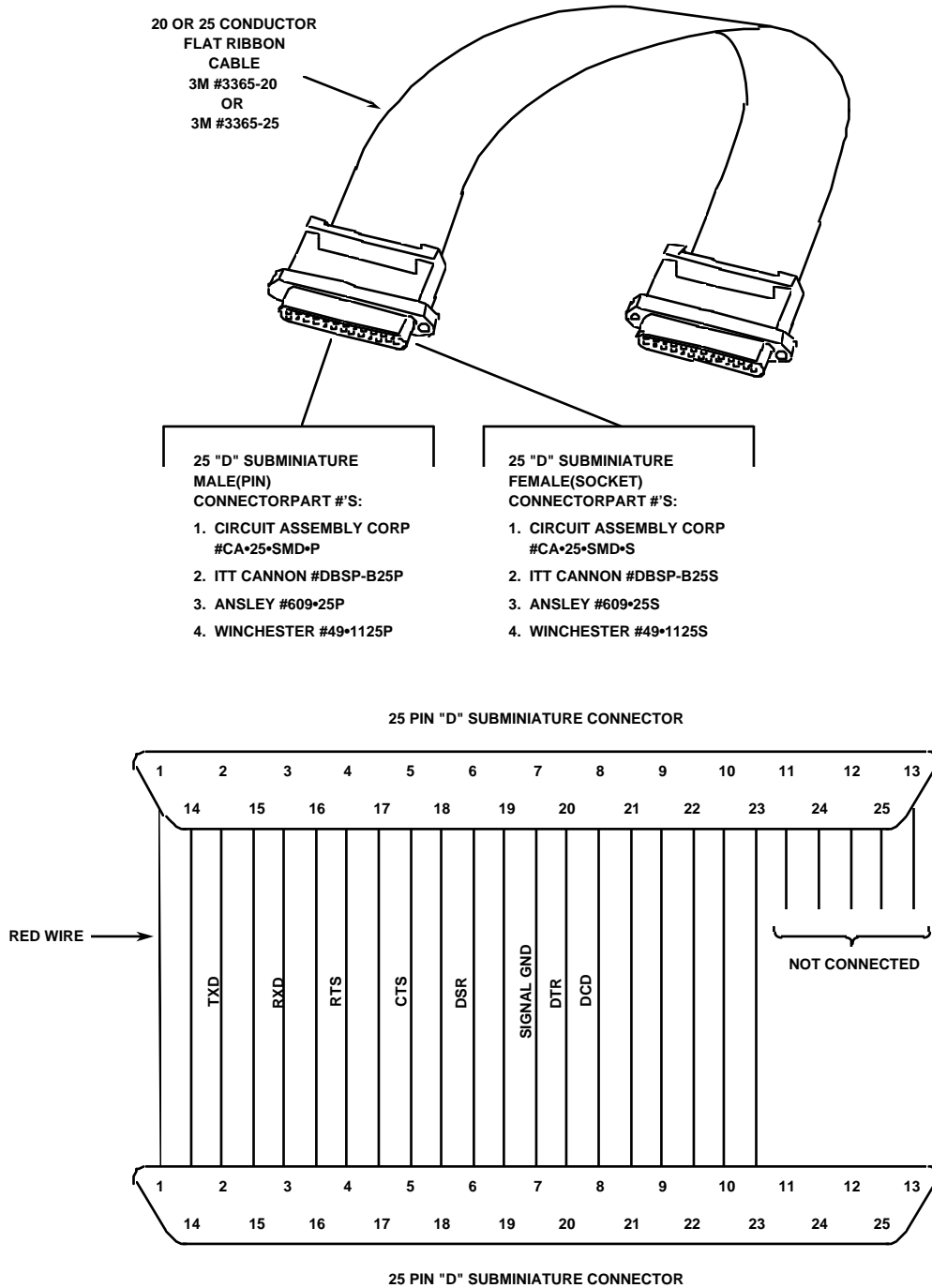
Figure 2-5. Terminal/Host Computer Cable Assembly Diagram
