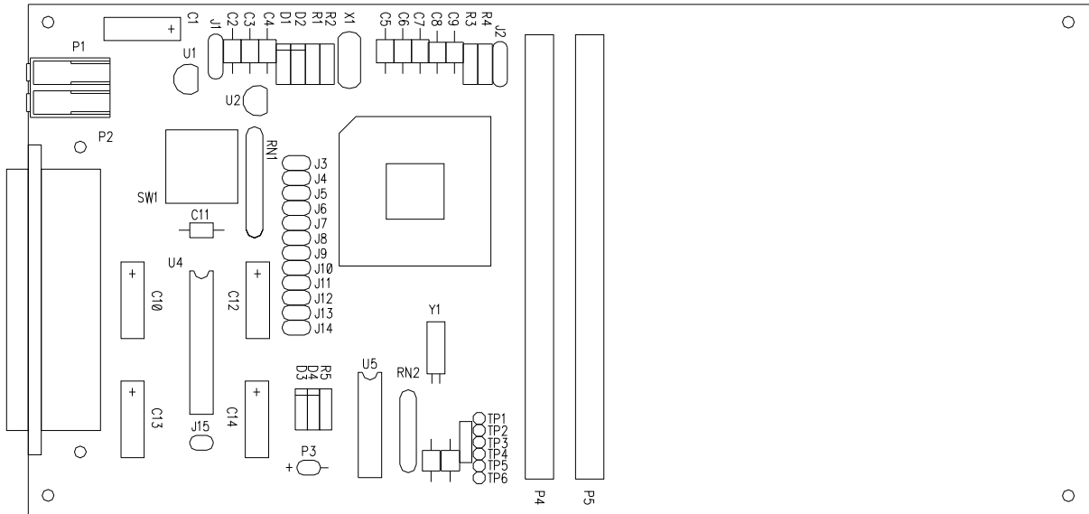
Figure 6-1. EVBU Parts Location Diagram
