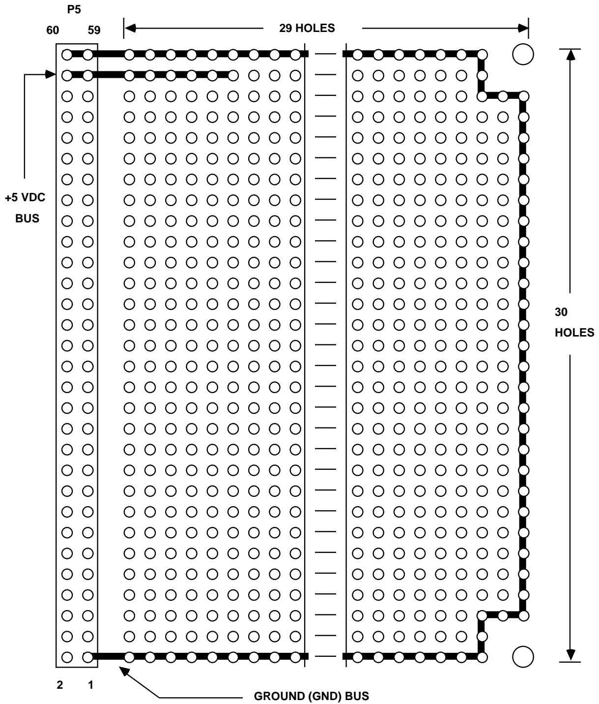
Figure 2-2. Wire-Wrap Area (Top Exploded View)
