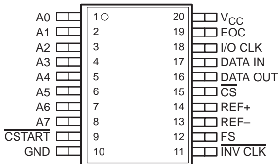
DB PACKAGE (TOP VIEW)
