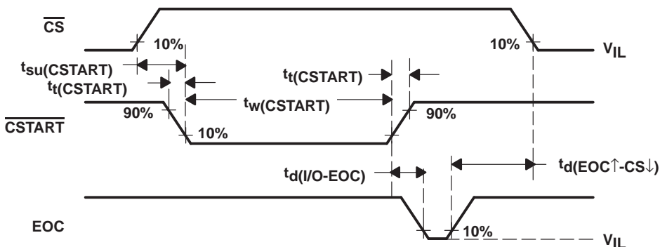
Figure 15. \overline{CSTART} and \overline{CS} Waveforms
