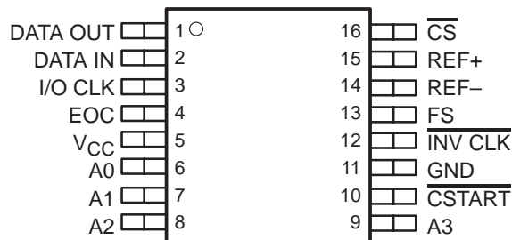
DB PACKAGE (TOP VIEW)
