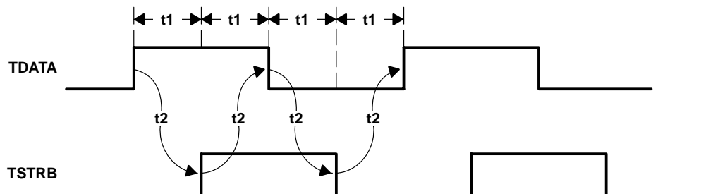
Figure 9. Minimum Edge Separation
