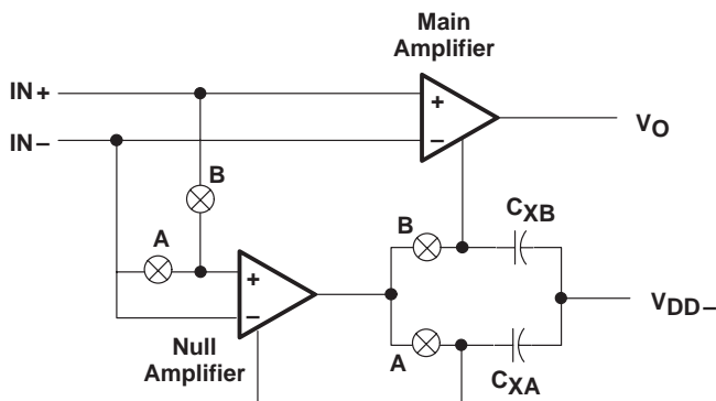
Figure 34. TLC2652 Simplified Block Diagram
