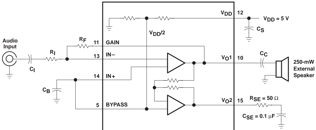
Figure 38. Single-Ended Mode
