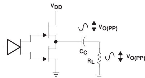
Figure 35. Single-Ended Configuration
