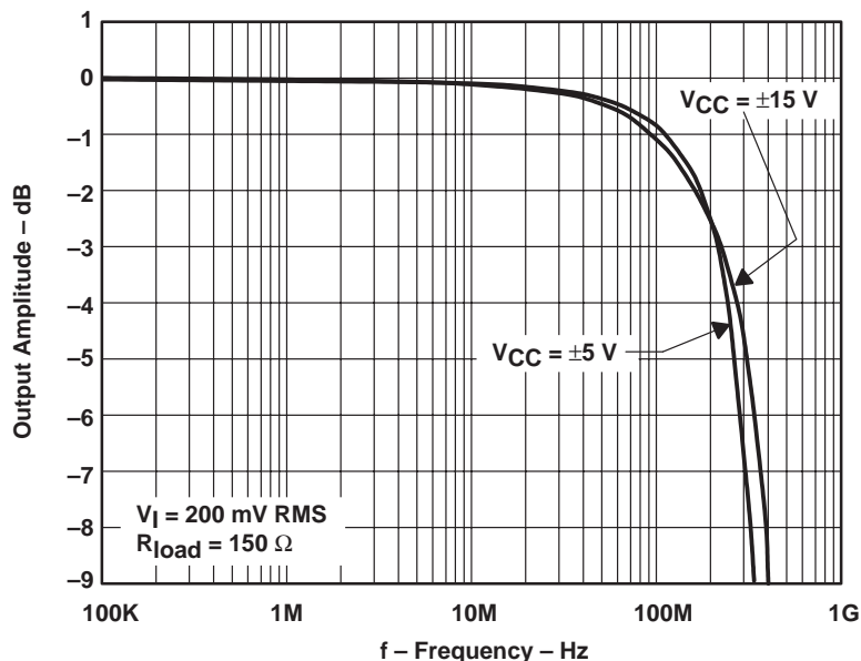
Figure 1–4. THS3001 EVM Frequency Response with Inverting Gain = 1
