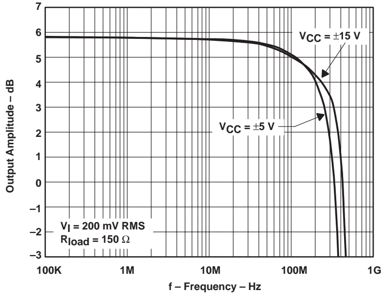
Figure 1–3. THS3001 EVM Frequency Response with Gain = 2
