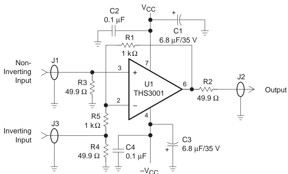
Figure 1–2. THS3001 EVM Schematic
