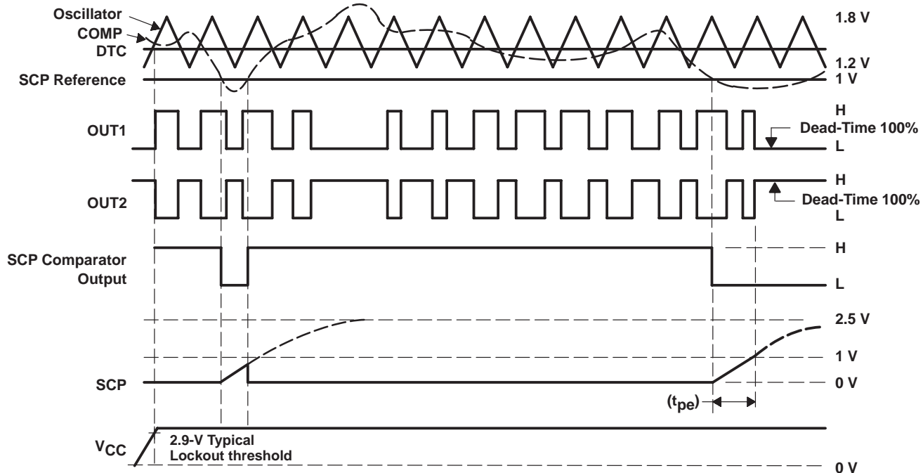
Figure 5. Timing Diagram
