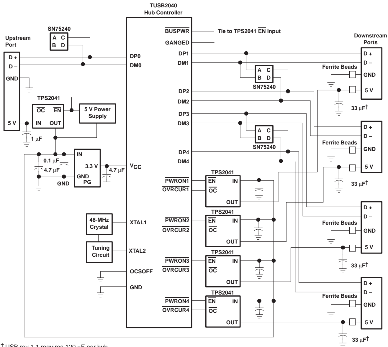
Figure 37. Hybrid Self/Bus-Powered Hub Implementation
