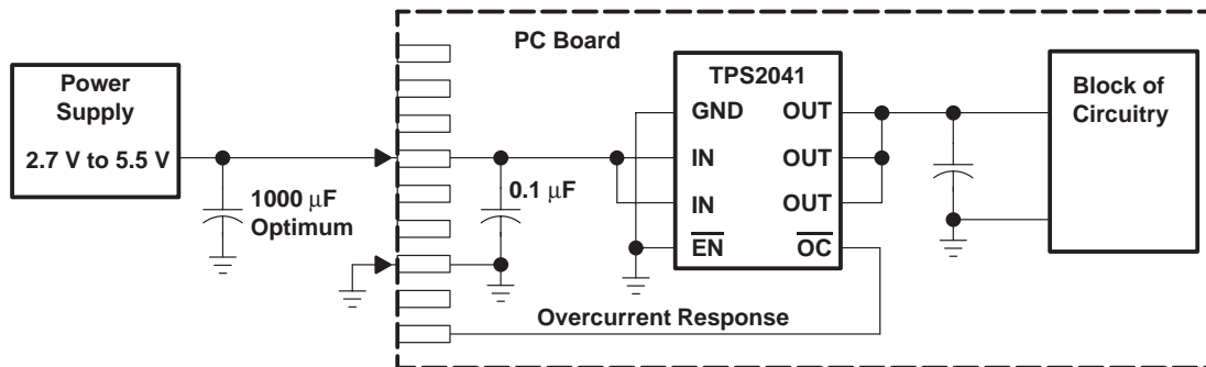
Figure 38. Typical Hot-Plug Implementation
