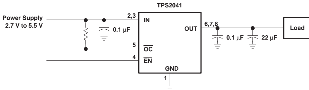
Figure 33. Typical Application
