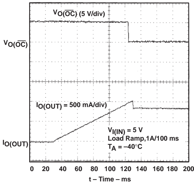
Figure 10. Ramped Load on Enabled Device
