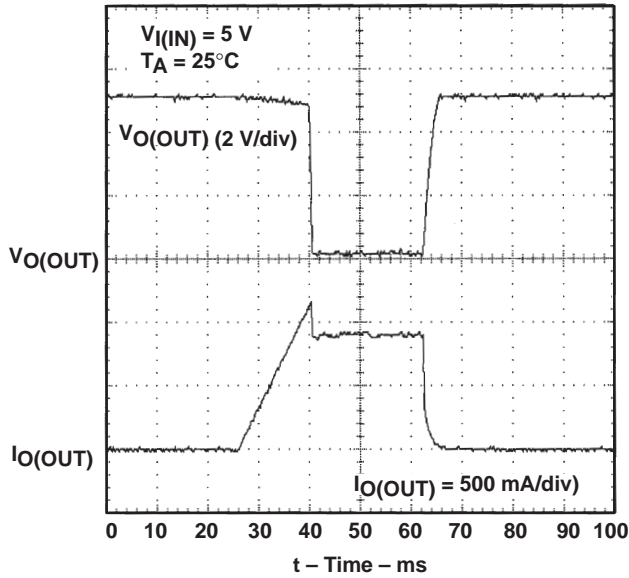
Figure 8. TPS2041, Threshold Trip Current with Ramped Load on Enabled Device
