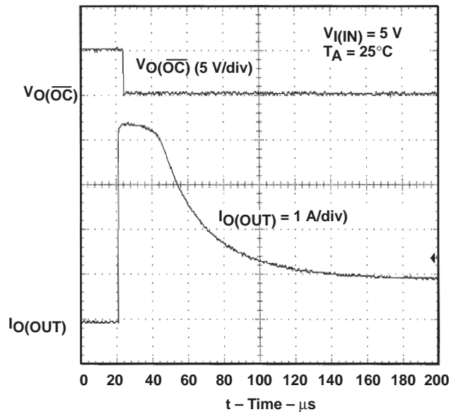
Figure 15. 1-Ω Load Connected to Enabled Device
