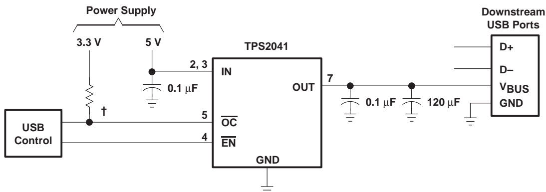
Figure 35. One-Port Solution
