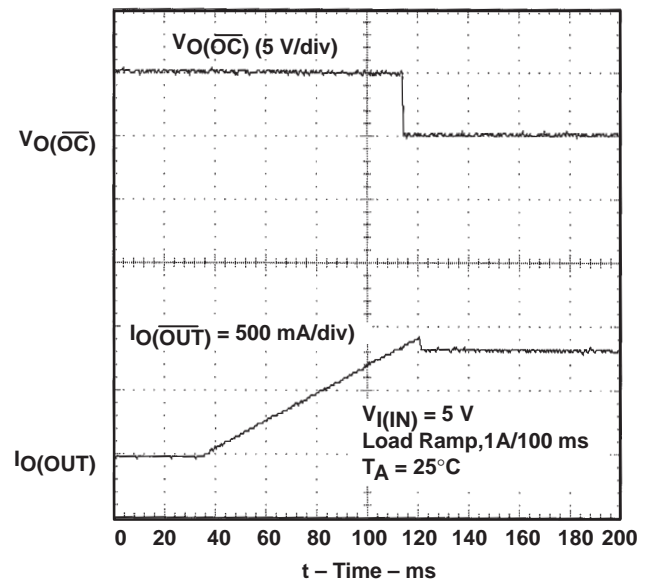
Figure 11. Ramped Load on Enabled Device
