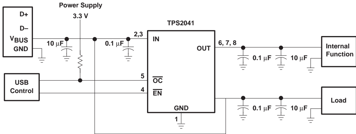
Figure 36. High-Power Bus-Powered Function
