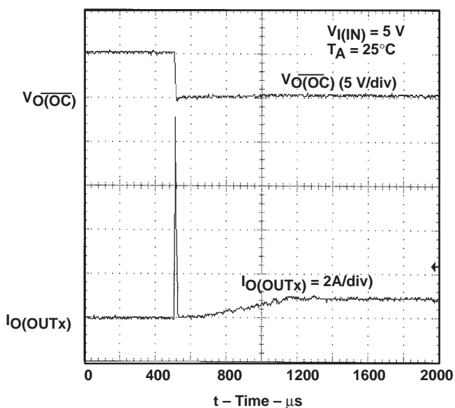
Figure 7. TPS2041, Short Connected to Enabled Device
