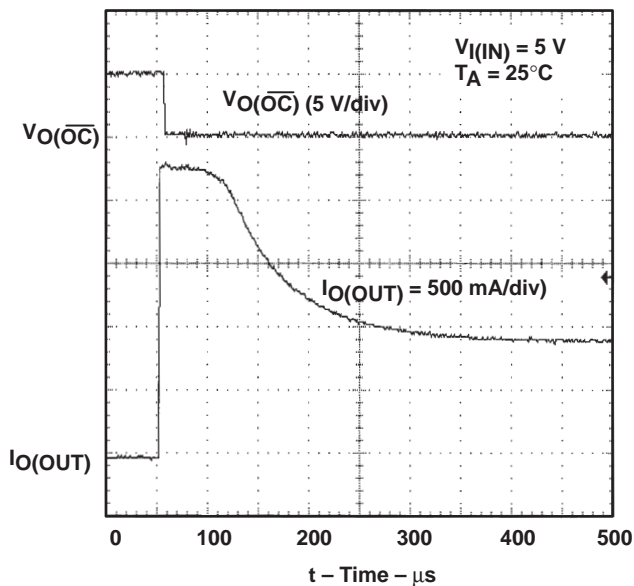
Figure 14. 2-Ω Load Connected to Enabled Device
