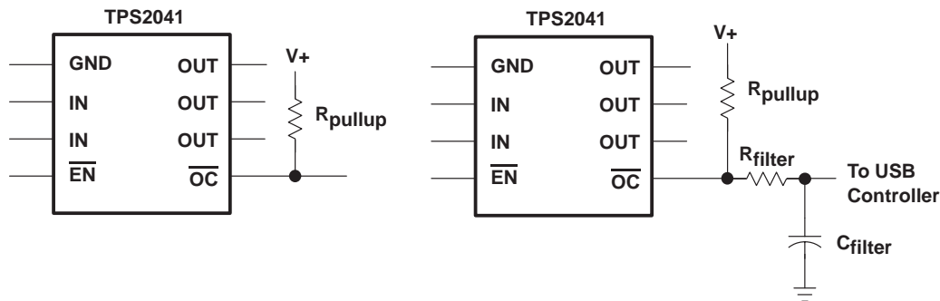
Figure 34. Typical Circuit for \overline{OC} Pin and RC Filter for Damping Inrush \overline{OC} Responses
