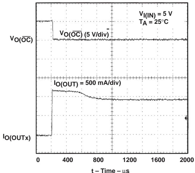
Figure 13. 4-Ω Load Connected to Enabled Device
