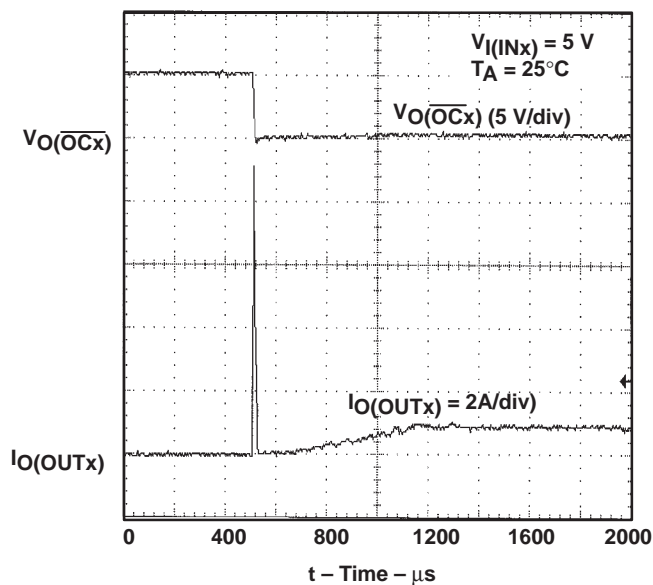
Figure 7. TPS2044, Short Connected to Enabled Device
