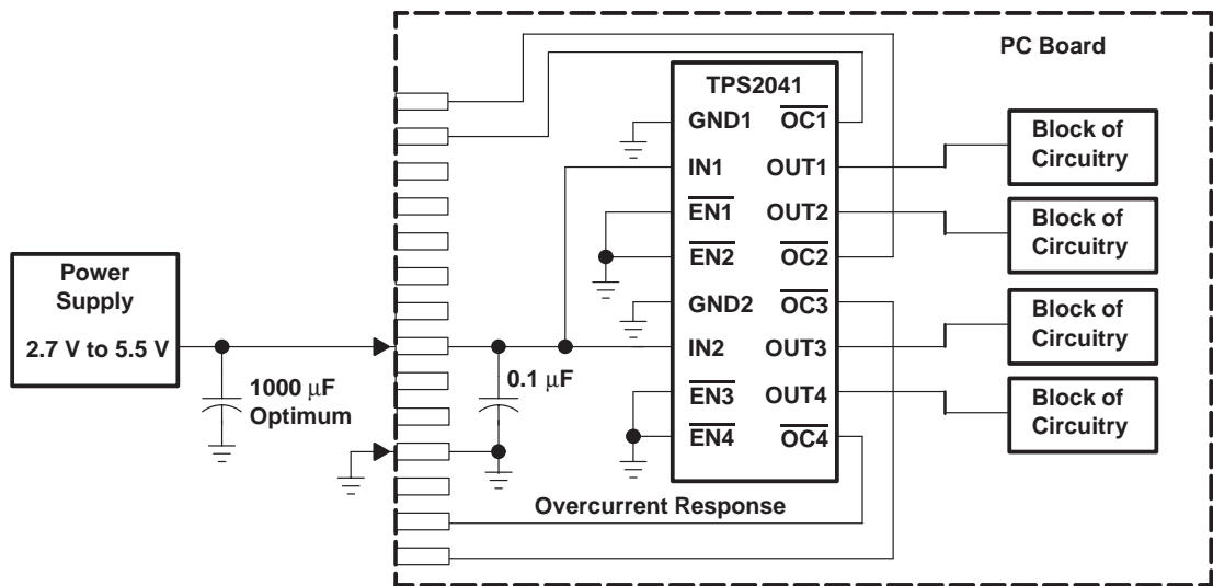
Figure 40. Typical Hot-Plug Implementation
