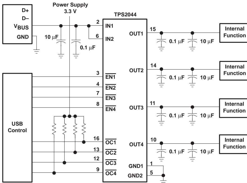
Figure 38. High-Power Bus-Powered Function
