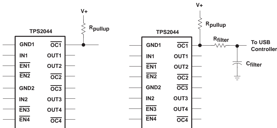
Figure 36. Typical Circuit for \overline{OC} Pin and RC Filter for Damping Inrush \overline{OC} Responses
