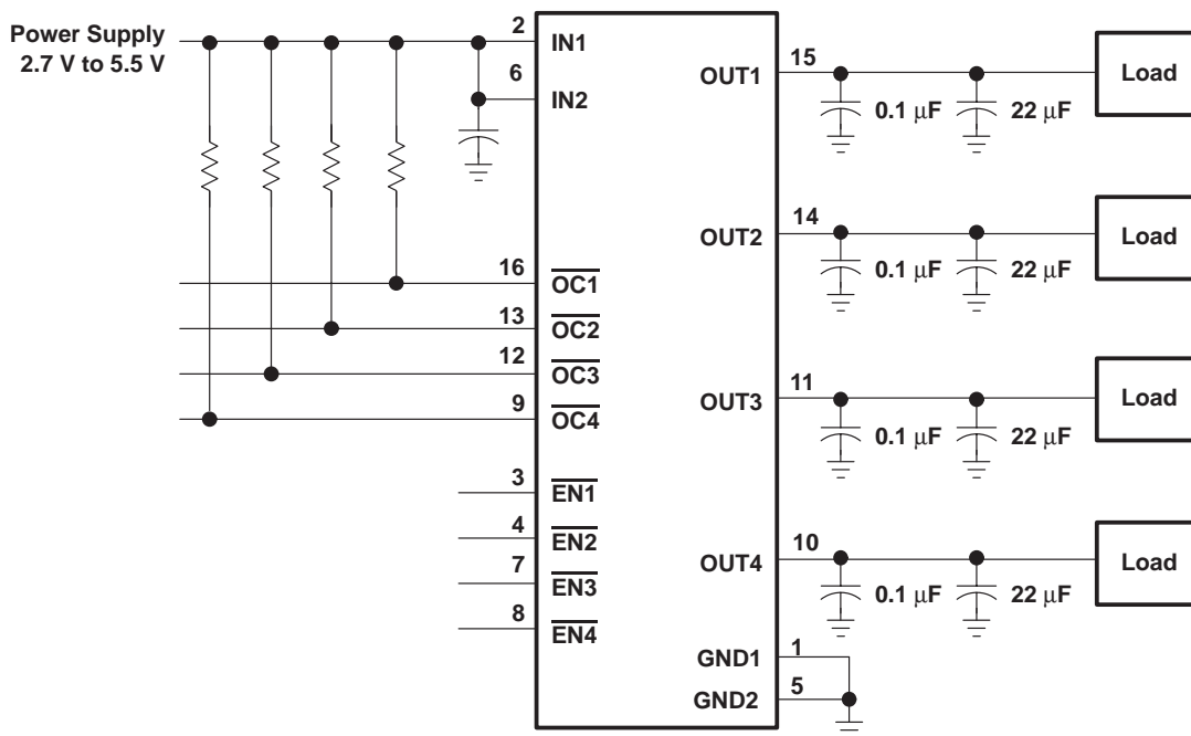
Figure 35. Typical Application
