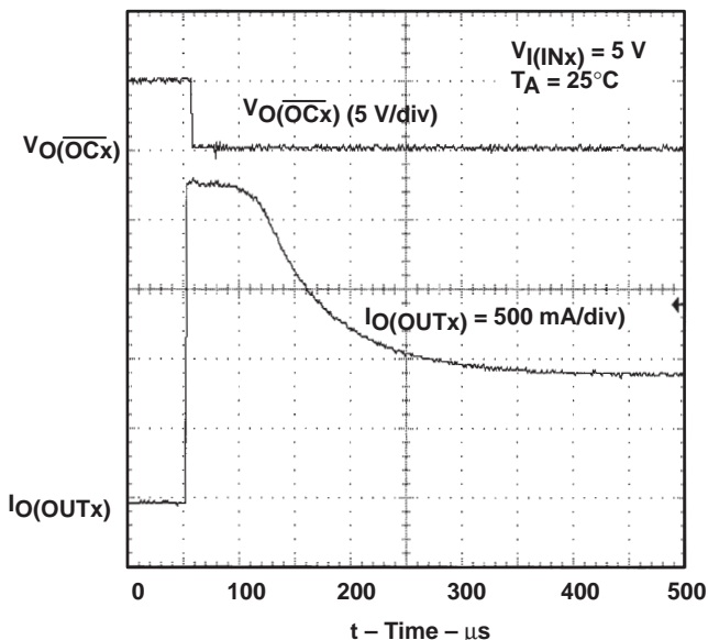
Figure 16. 2-Ω Load Connected to Enabled Device
