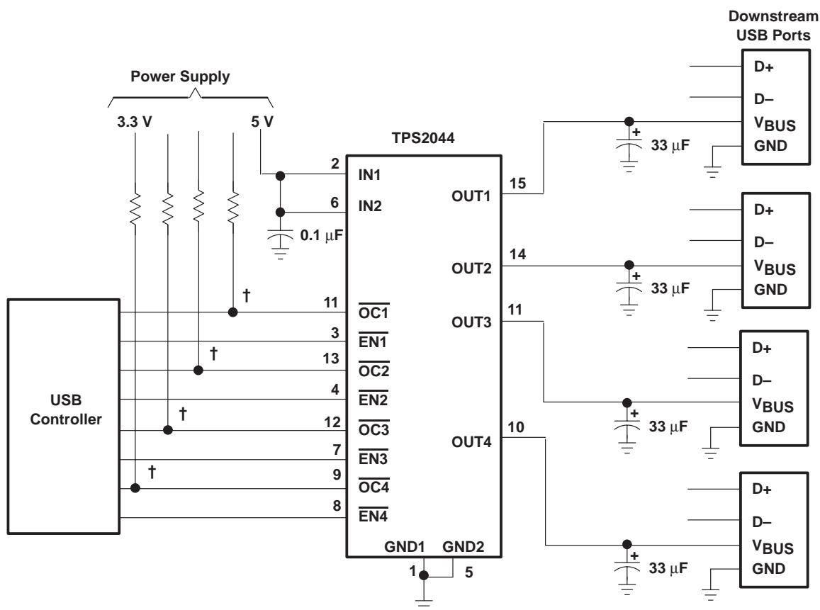
Figure 37. Typical Four-Port USB Host/Self-Powered Hub
