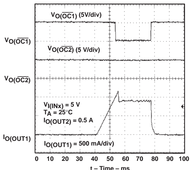
Figure 9. TPS2044, \overline{OC1} and \overline{OC2} Response with Ramped Load on OUT1 and Fixed Load on OUT2
