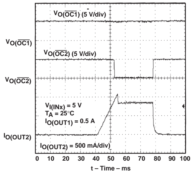
Figure 10. TPS2044, \overline{OC1} and \overline{OC2} Response with Ramped Load on OUT2 and Fixed Load on OUT1
