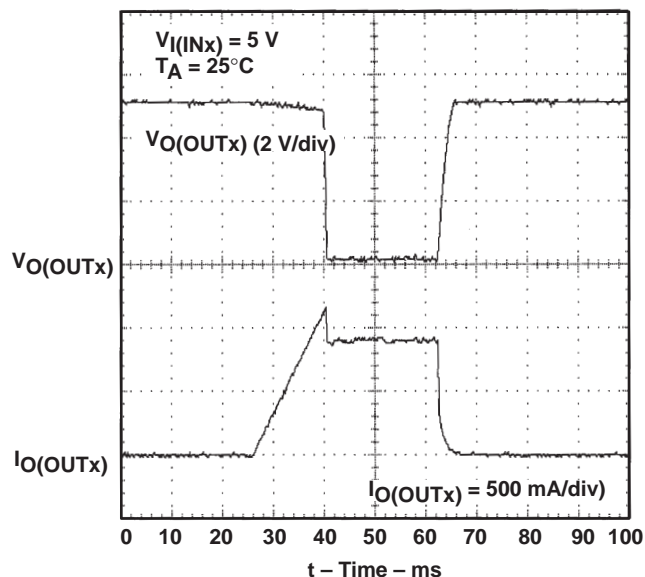
Figure 8. TPS2044, Threshold Trip Current with Ramped Load on Enabled Device
