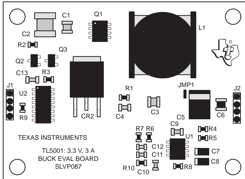
Figure 1–4. Board Layout
