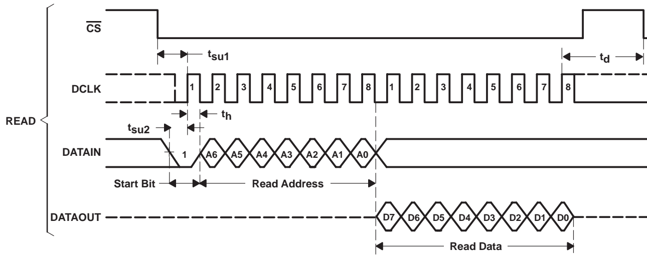
Figure 3-2. Microcontroller Interface Read Timing Diagram
