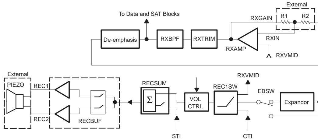
Figure 5–2. Receive Audio Path
