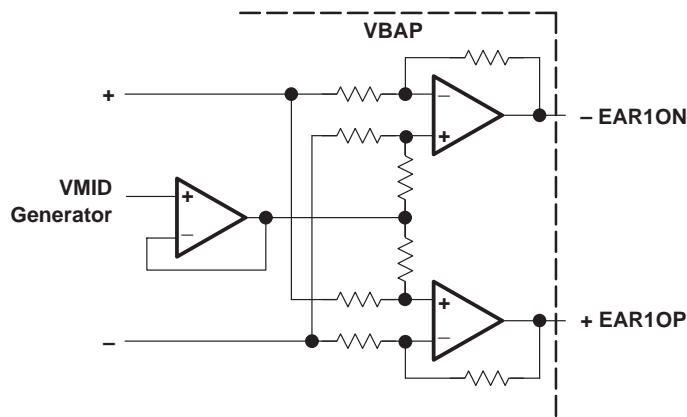
Figure 6. Differential Earphone Amplifier Configuration
