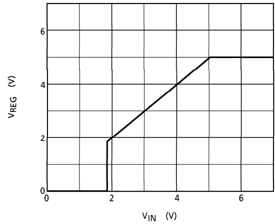
INPUT-OUTPUT CHARACTERISTICS
