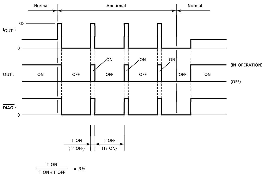
SELF DIAGNOSIS TIMING CHART
