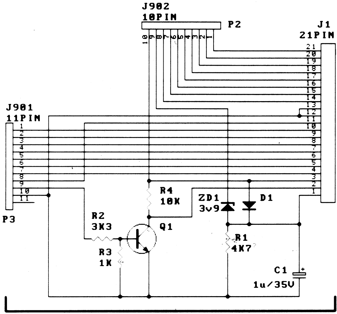
ADAPTOR PCB
