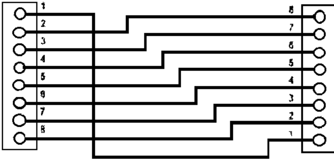
Cable (figure 2)
