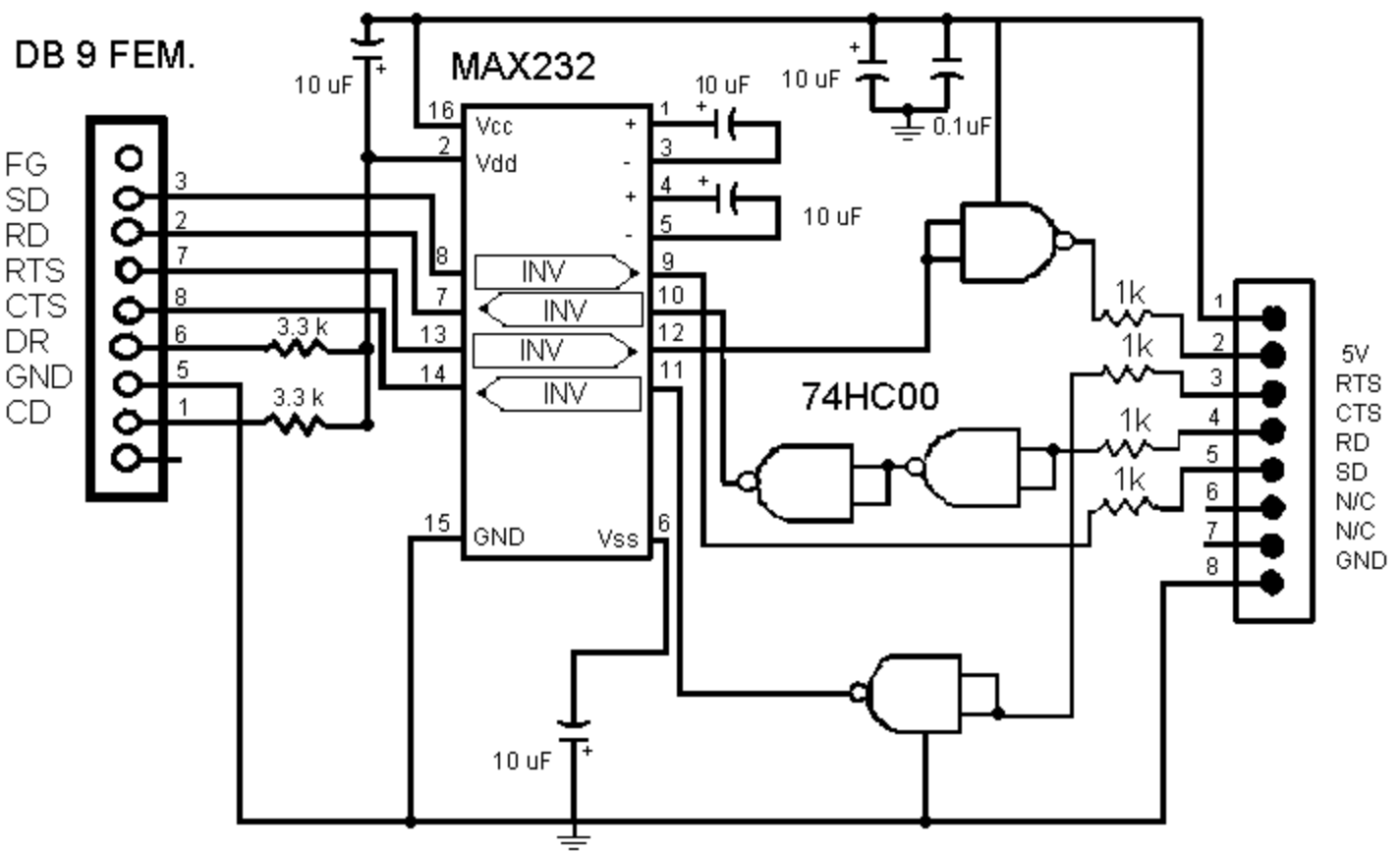
Cable (figure 2)
