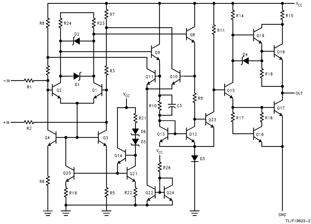
FIGURE 1. Equivalent Circuit
