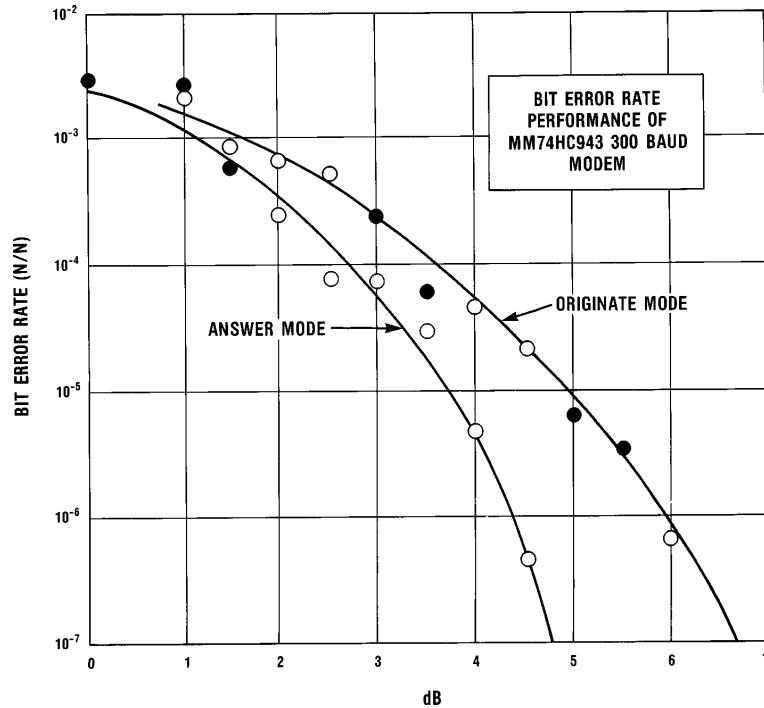
FIGURE 16. Bit Error Rate Performance of MM74HC943 300 Baud Modem
