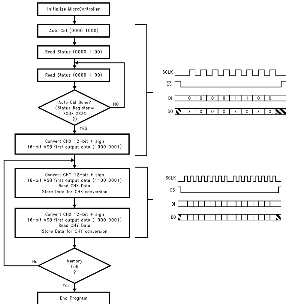
FIGURE 3. ADC12038 Program Flow Chart and Timing
