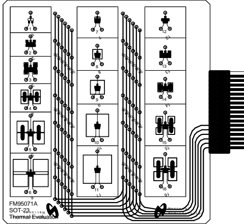
Figure 2. Top Side of the 4.5''x5'' SuperSOT™-3 Thermal Board. Complete scale drawings is shown in appendix D.
