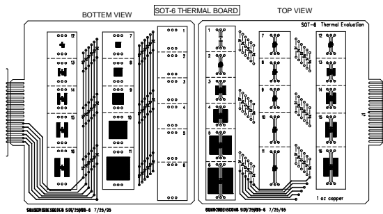
Figure 2. Both Sides of the 4.5"x5" SuperSOT™-6 Thermal Board. Complete scale drawings is shown in appendix D.
