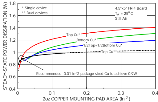
Figure 4. Maximum Power Dissipation Curves for SuperSOT™-6. For single device, layout 2 0.01 in² 2 Oz copper mounting pad area is recommended to achieve approximately 0.9W.
