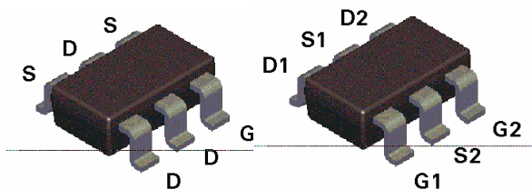
Figure 1. SuperSOT™-6 Power MOSFET achieves junction-to-case thermal resistance R_{\theta JC} of 30°C/W for single device and 60°C/W for dual devices.
