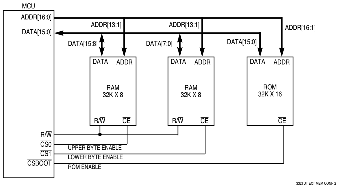
Figure 13 Configuring 16-Bit Memory with 8-Bit RAMs — Common R/W Input
