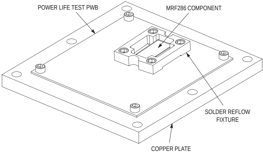
Figure 3. MRF286 Component Assembled with Solder Reflow Fixture
